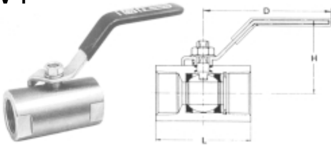
Ball Valve (Reducing Bore) 800 WOG SV-1
