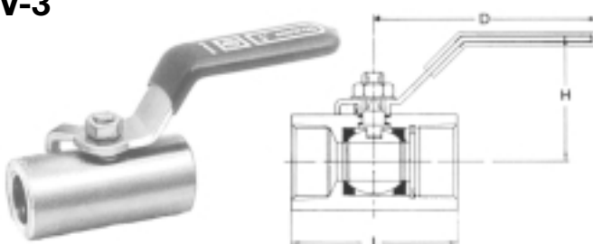
Miniature Ball Valve (Reducing Bore) 800 WOG SV-3
